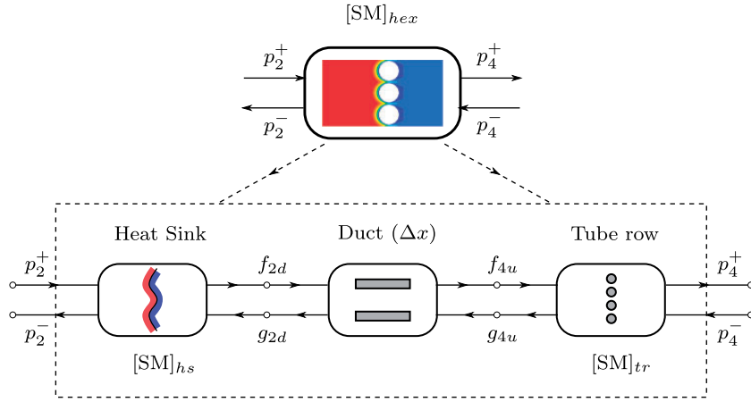
Figure 6. Schematic of the network modelling approach used on hex.
