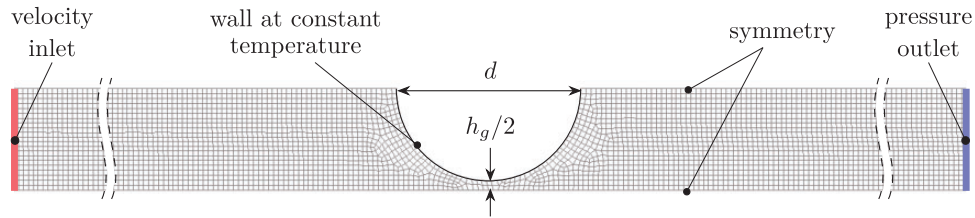
Figure 3. Meshed geometry with boundary conditions.
