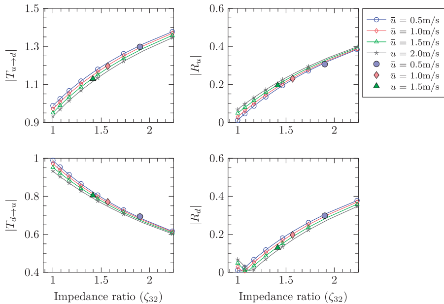
Figure 8. Variation of the elements of [SM]_{hex} as a function of \zeta_{32} , for fixed velocities, f=100 Hz, d=3 mm and \eta=0.1 . Solid markers indicate the results obtained by including \alpha and curves indicate the results obtained by using \alpha=0 .
