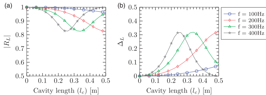
Figure 9. Variation of |R_L| and \Delta_L as functions of the cavity length ( l_c ), for fixed frequencies, d = 3 mm, \eta = 0.1 , \zeta_{32} = 1.936 , R_p = 1 and \bar{u} = 2.0 m/s.
