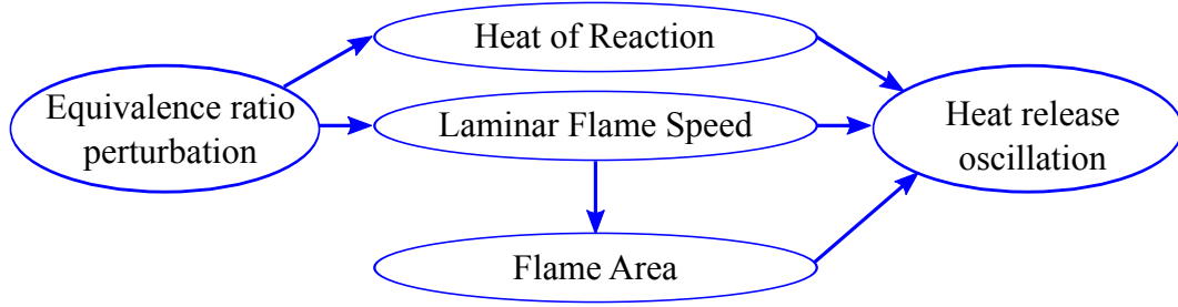
Figure 1. Major mechanisms causing heat release rate oscillations [5]
