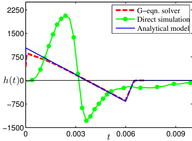
Figure 5. Validation study of impulse response
