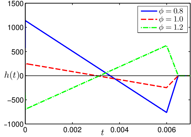
Figure 6. Impulse responses for different mean equivalence ratios
