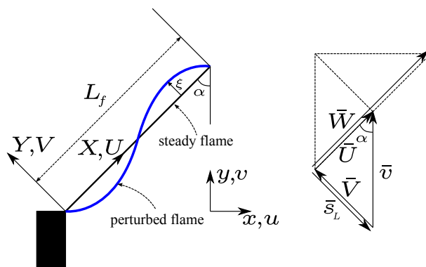
Figure 2. Flame-aligned coordinate system
