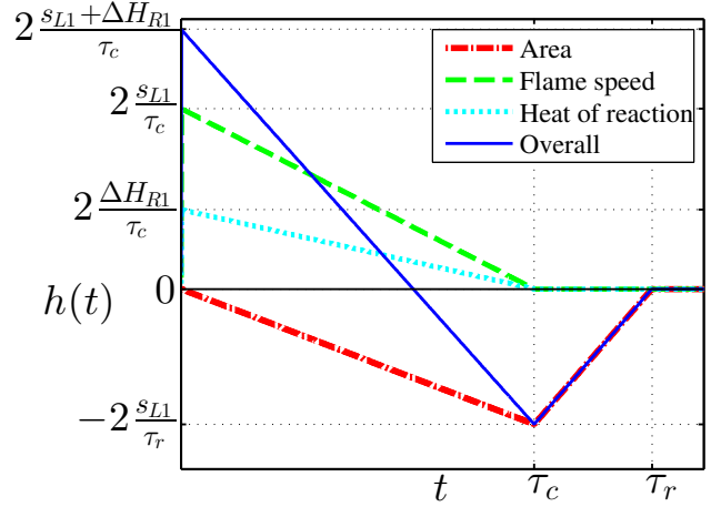
Figure 4. Impulse responses for each contribution
