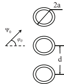
Figure 2: Geometry of the tube row.
